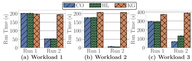
Figure 4: Repeated executions of Kaggle workloads
