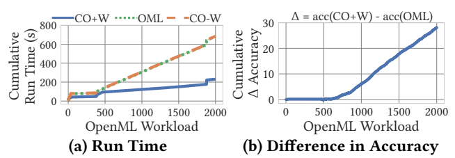
Figure 10: Warmstarting of OpenML workloads
