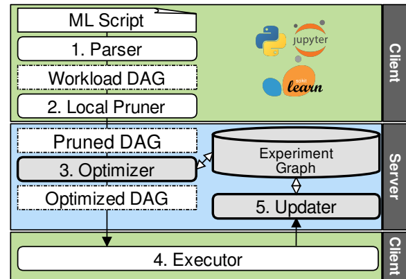
Figure 2: Collaborative workload optimizer system
