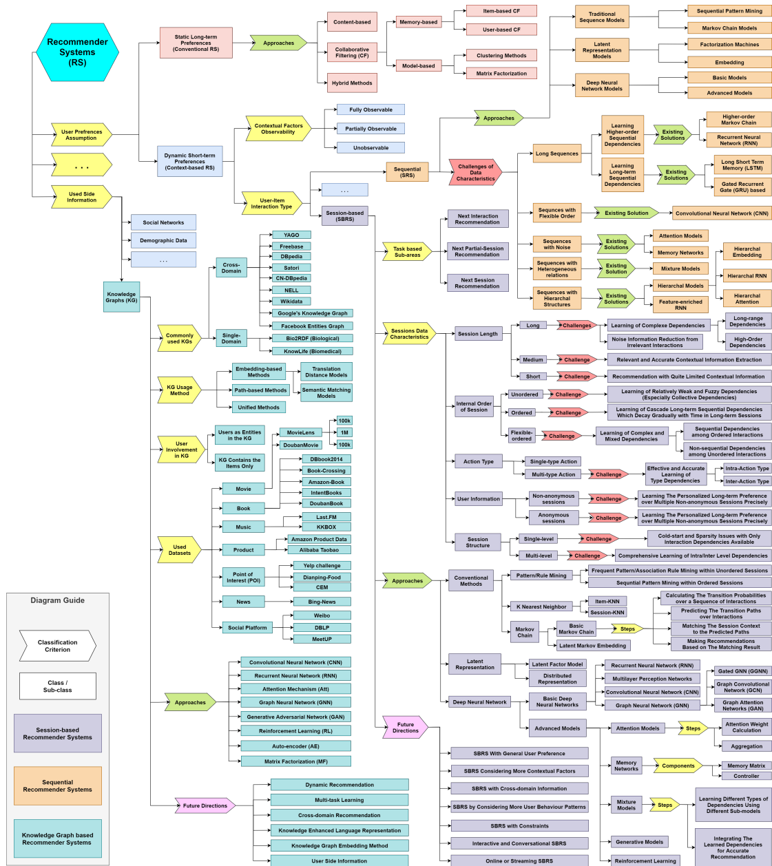
Figure 1: Recommender systems state of the art with focus on the three most relevant categories. (high-resolution version available online: https://www.dfki.uni-kl.de/~bakhshizadeh/lwda2021/ )
